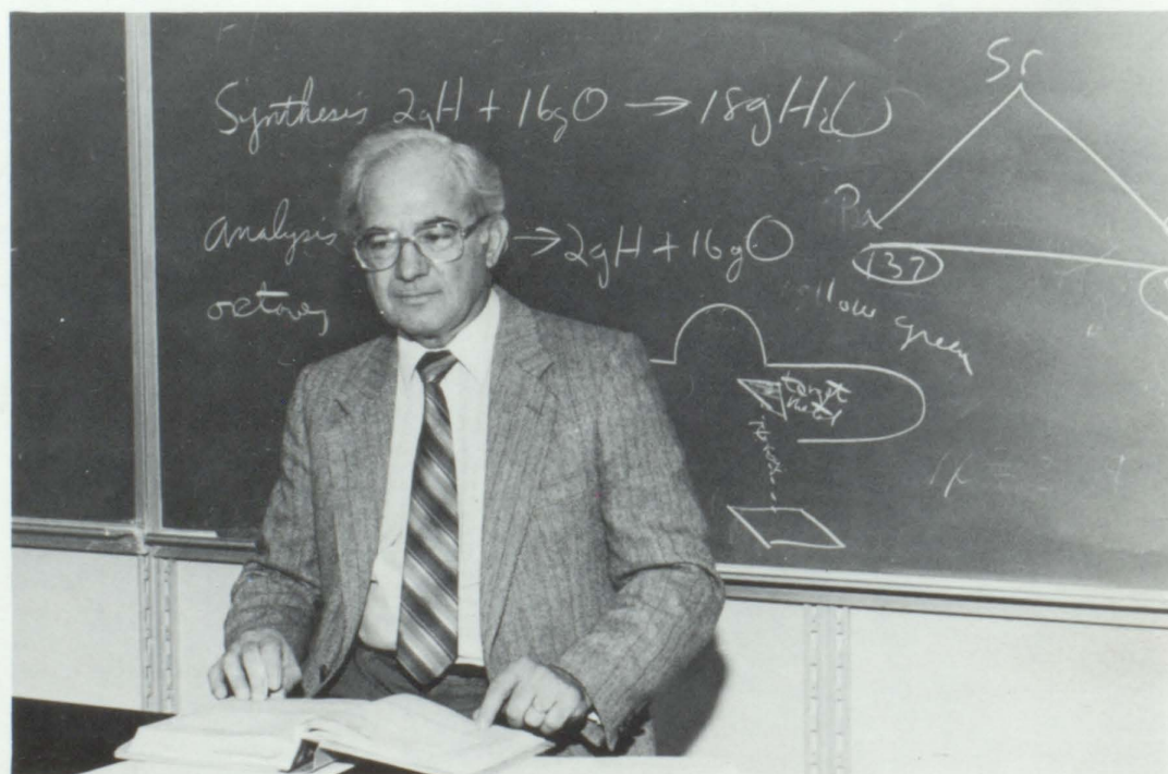
Mr. Rullo discussed the balanced equations with his chemistry class.
